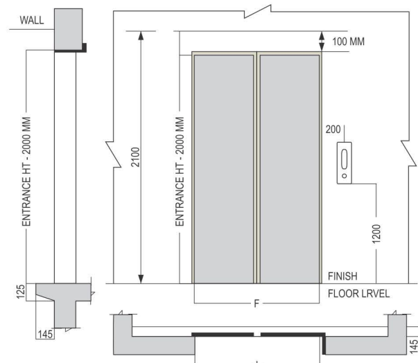
Details at Door Opening
